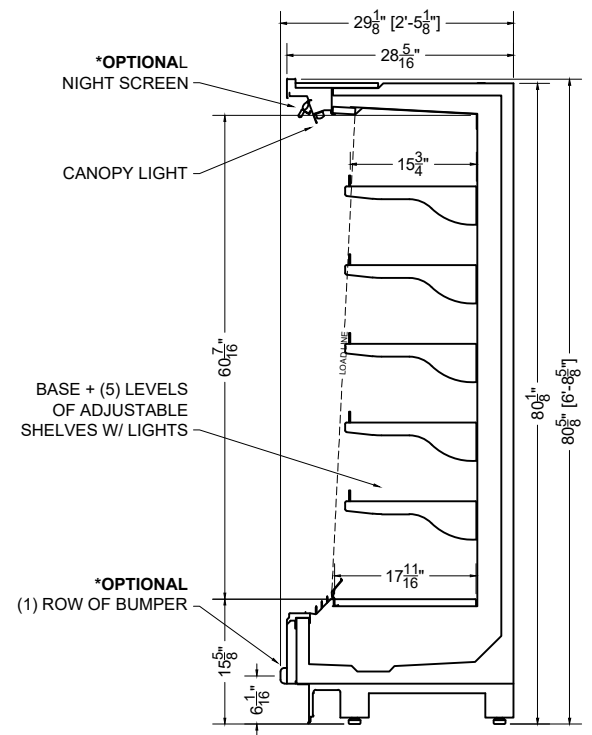
SECTION VIEW
