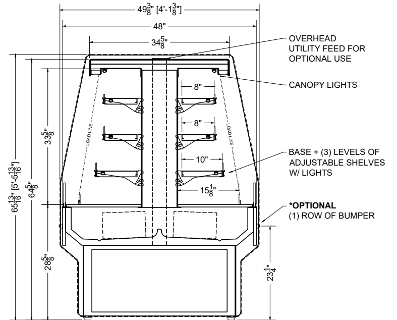
SECTION VIEW
