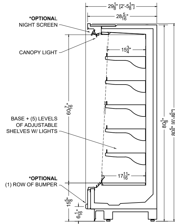
SECTION VIEW
