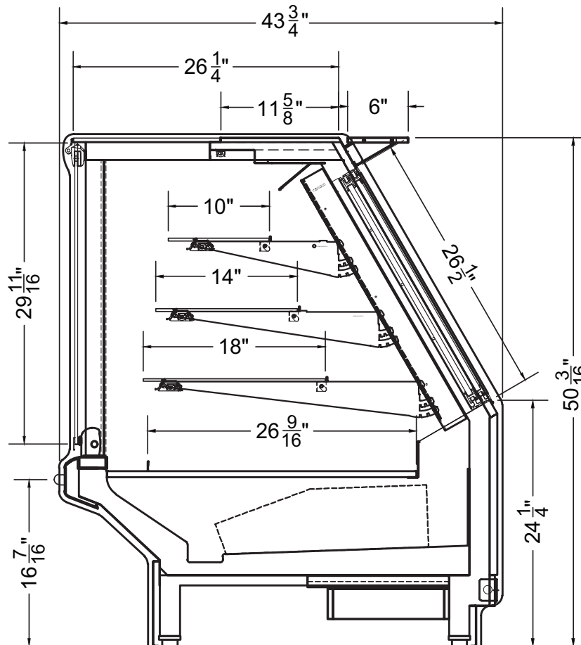
Section View
