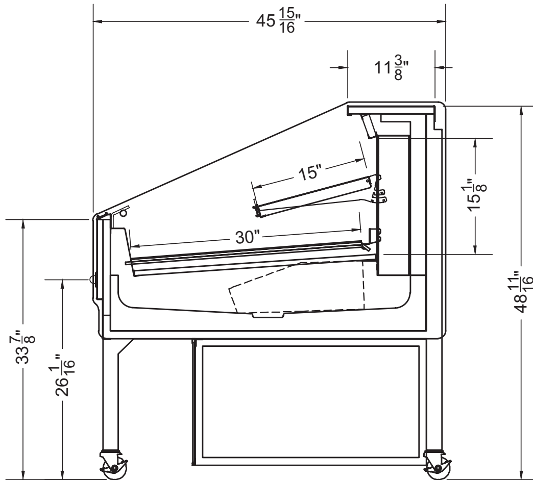
Section View
