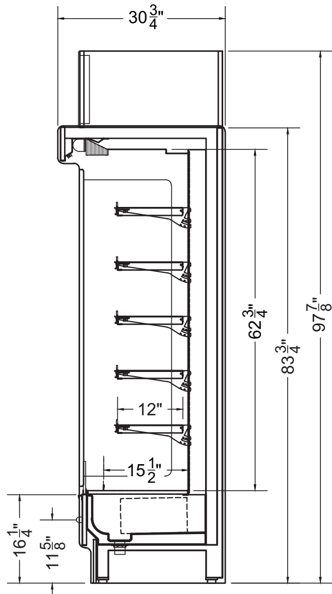
Section View
