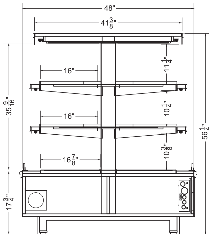
Section View
