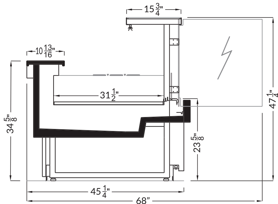
Section View
