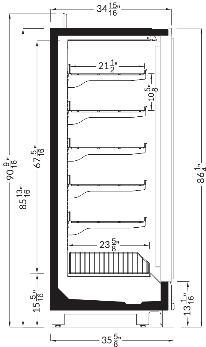
Section View
