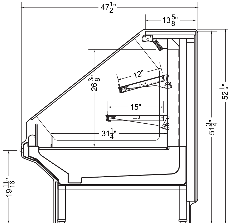
Section View
