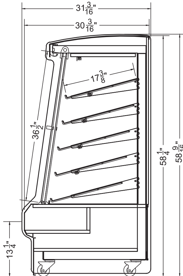
Section View
