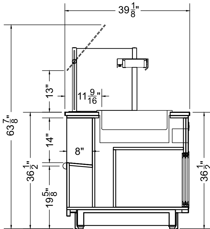
Section View
