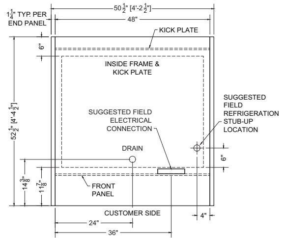
Plan Mechanical View
