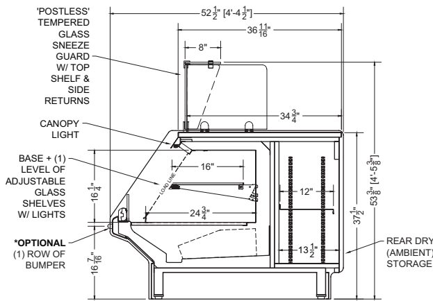
Section View
