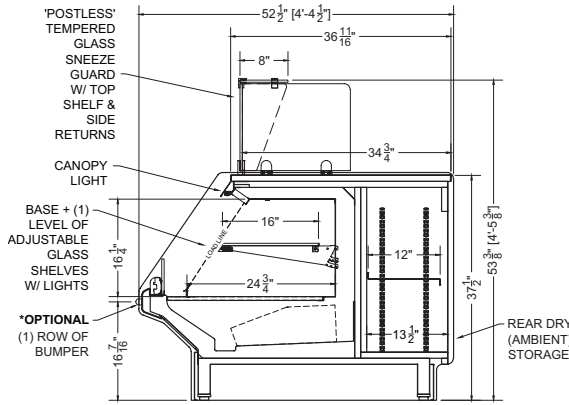
Section View
