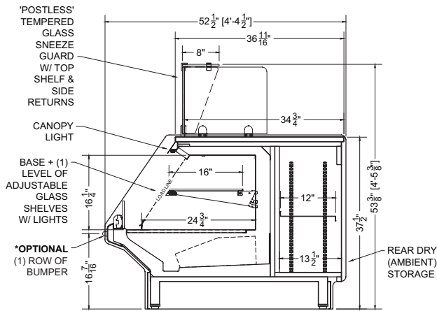
Section View
