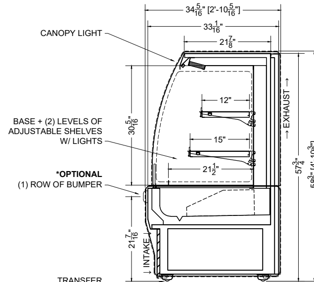
SECTION VIEW
