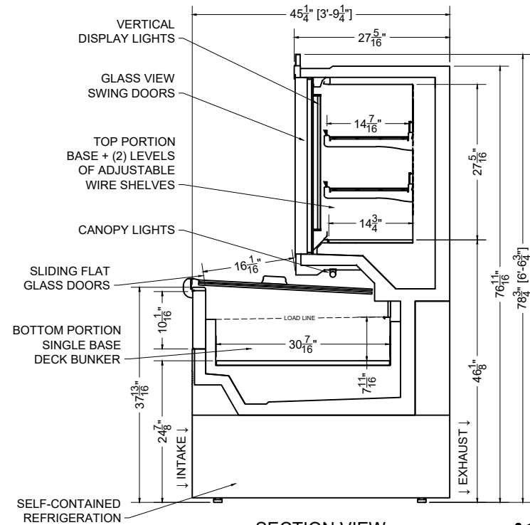
SECTION VIEW
