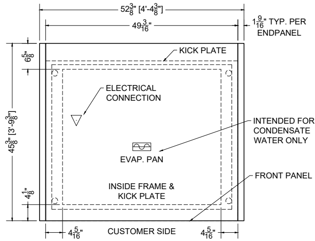
PLAN MECHANICAL VIEW
