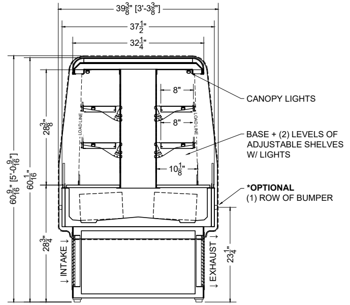
SECTION VIEW
