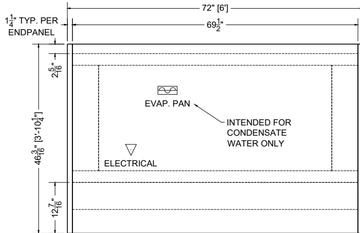
CUSTOMER SIDE PLAN MECHANICAL VIEW
