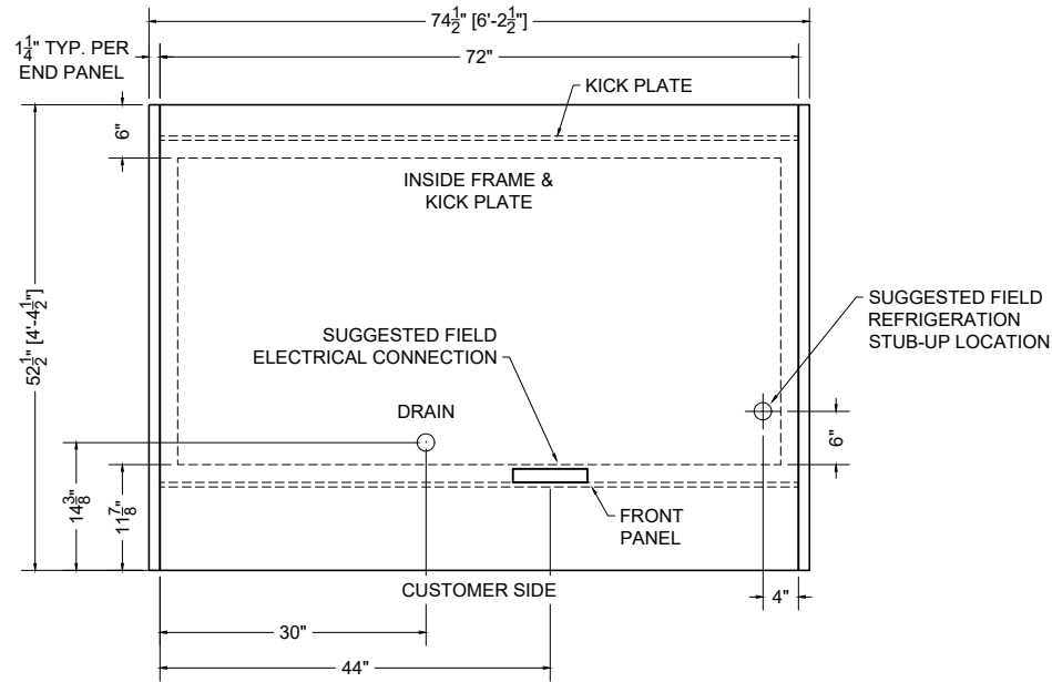
PLAN MECHANICAL VIEW
