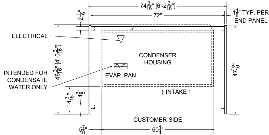
PLAN MECHANICAL VIEW
