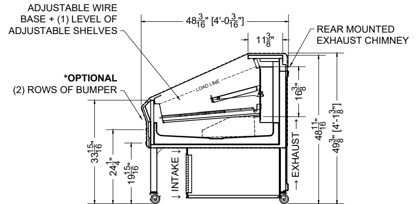
SECTION VIEW
