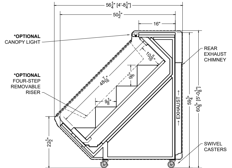
SECTION VIEW
