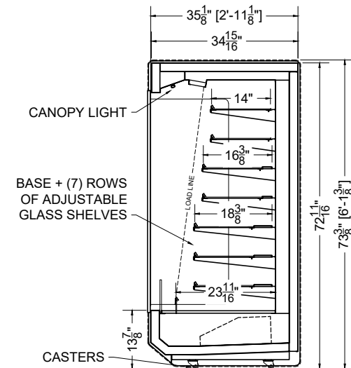
SECTION VIEW
