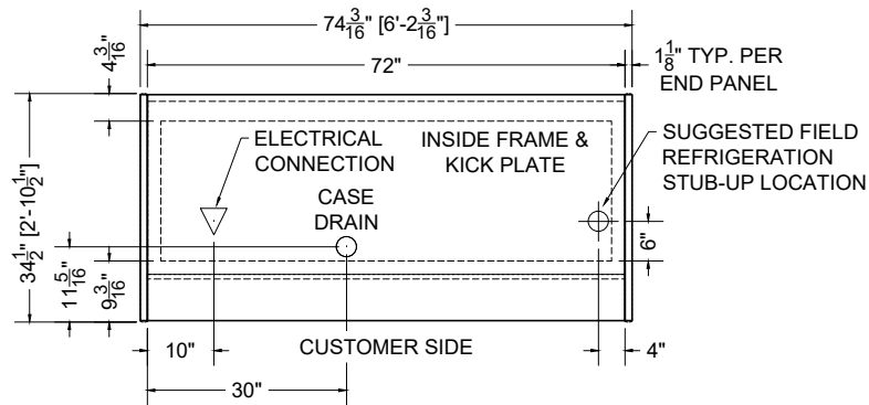
PLAN MECHANICAL VIEW
