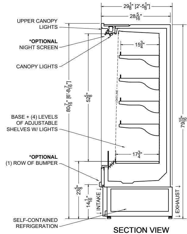
SECTION VIEW
