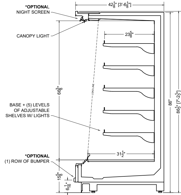
SECTION VIEW
