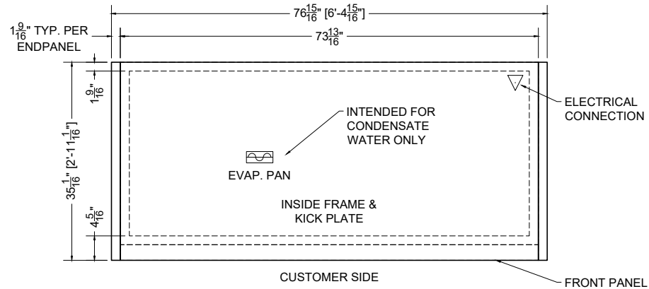
PLAN MECHANICAL VIEW
