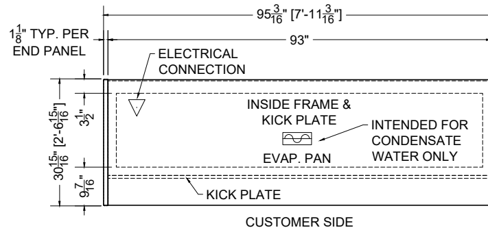
PLAN MECHANICAL VIEW
