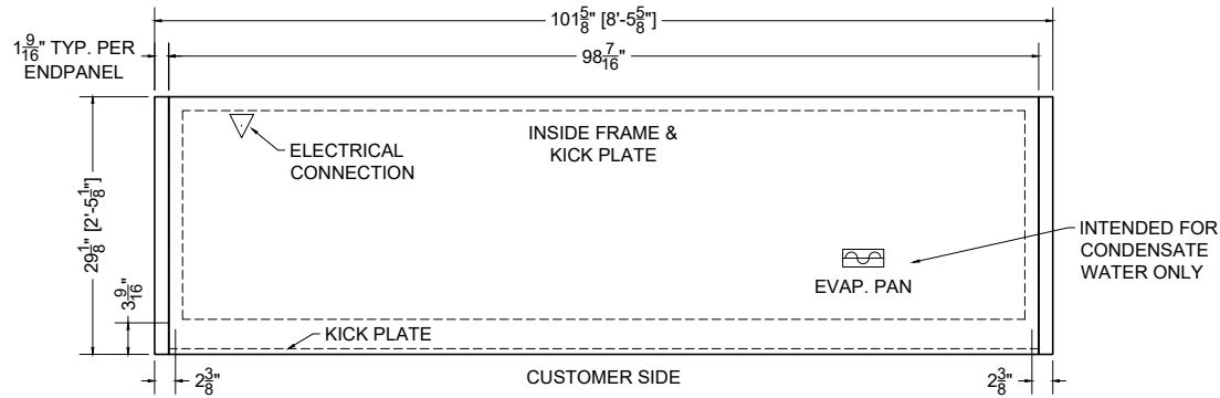
PLAN MECHANICAL VIEW
