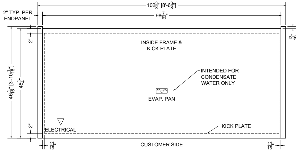
PLAN MECHANICAL VIEW
