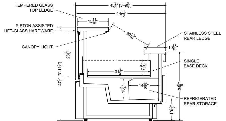
SECTION VIEW
