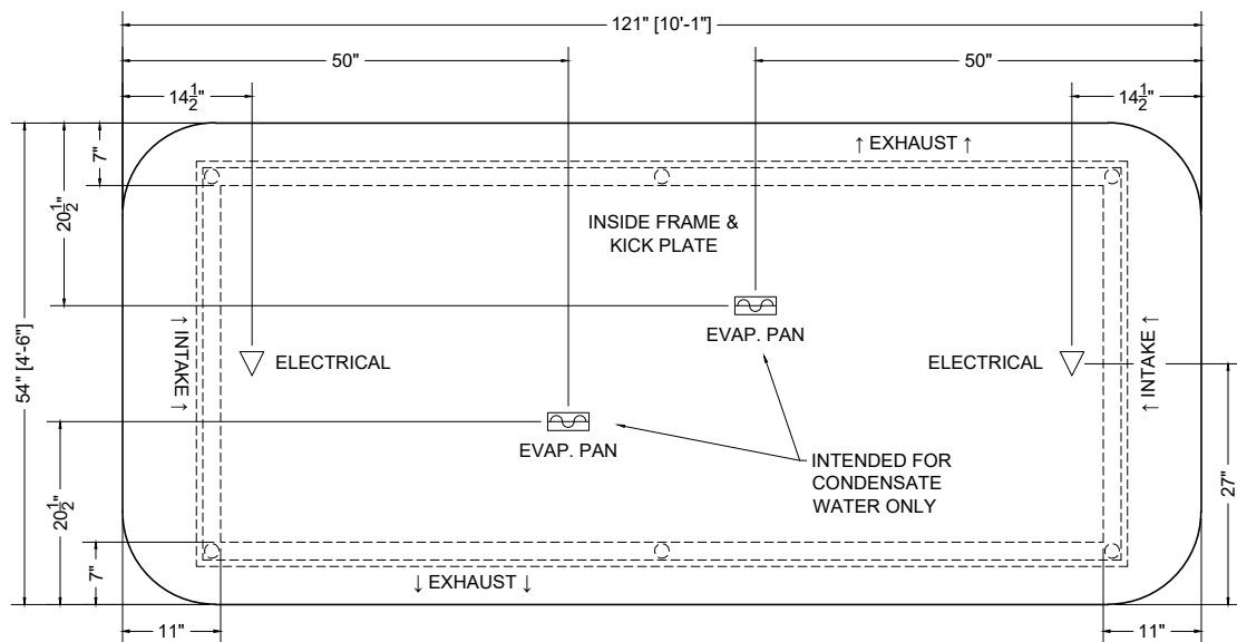
PLAN MECHANICAL VIEW
