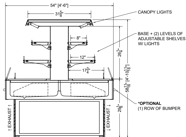
SECTION VIEW
