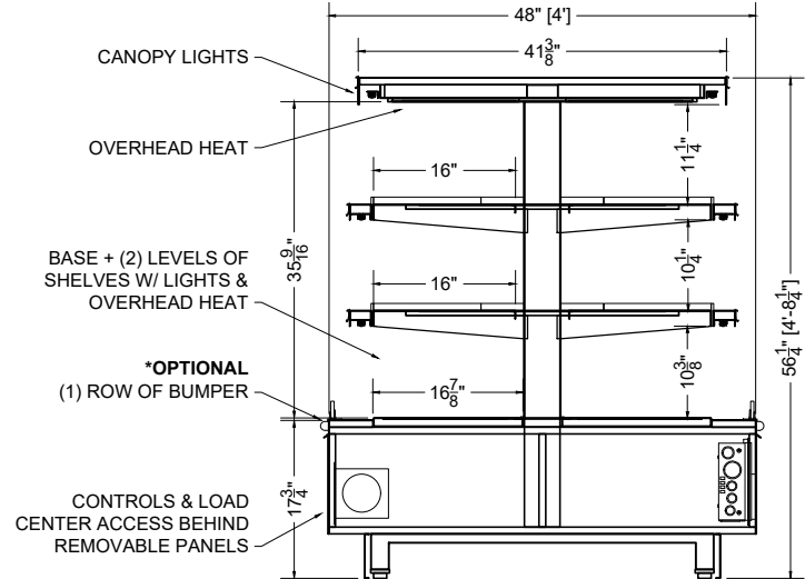
SECTION VIEW
