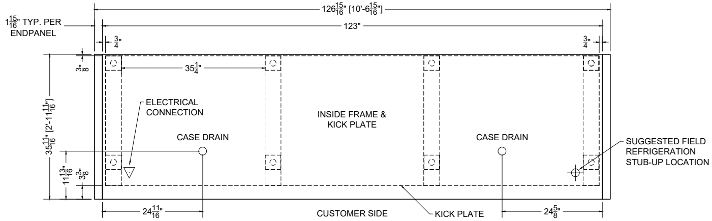
PLAN MECHANICAL VIEW
