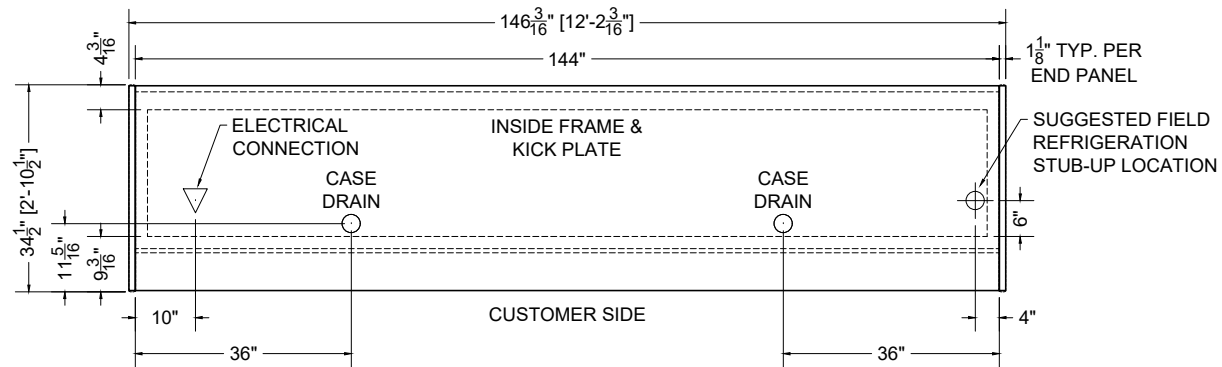
PLAN MECHANICAL VIEW
