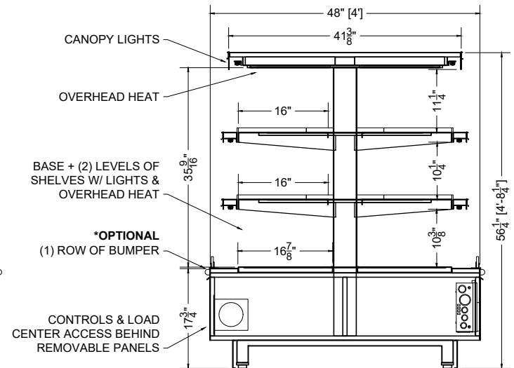
SECTION VIEW
