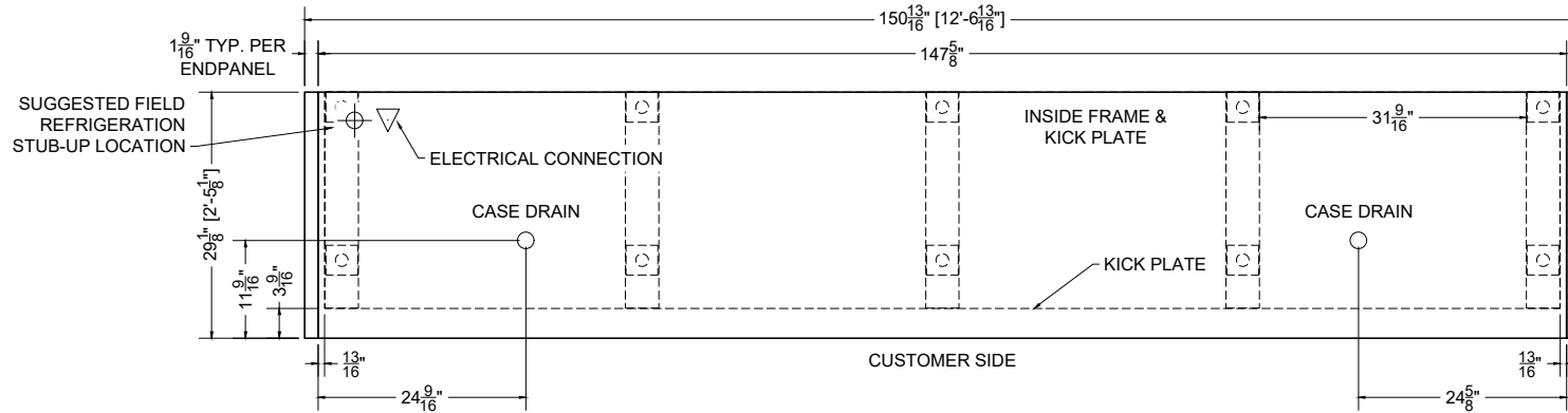
PLAN MECHANICAL VIEW
