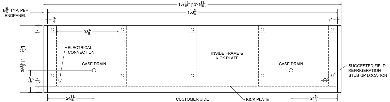
PLAN MECHANICAL VIEW
