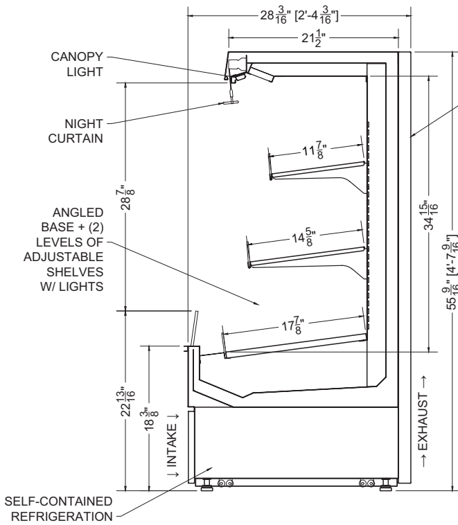
Plan Mechanical View
