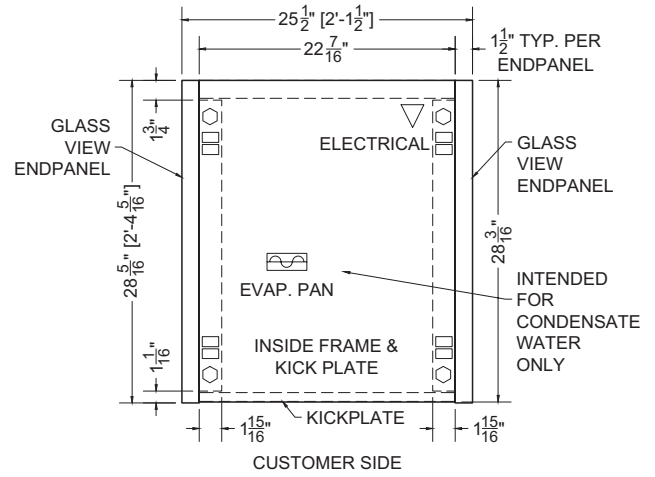
Section View
