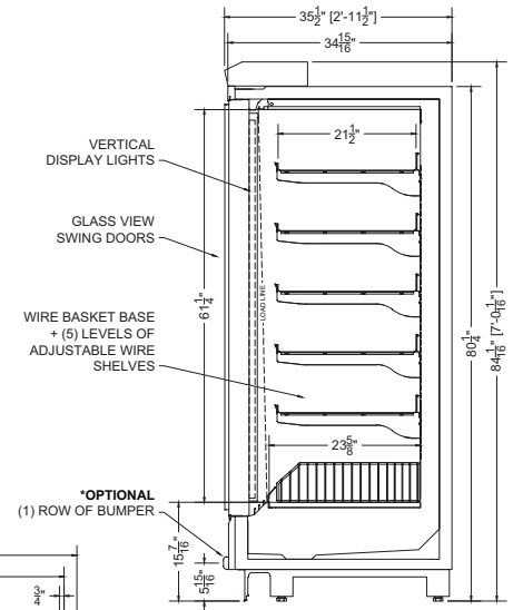
Section View
