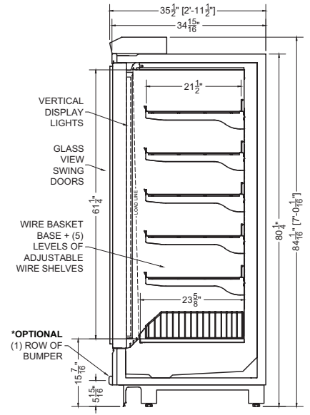
Section View
