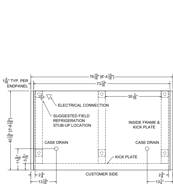
Plan Mechanical View
