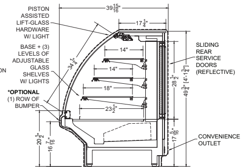
Section View
