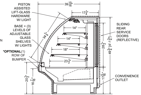
Section View
