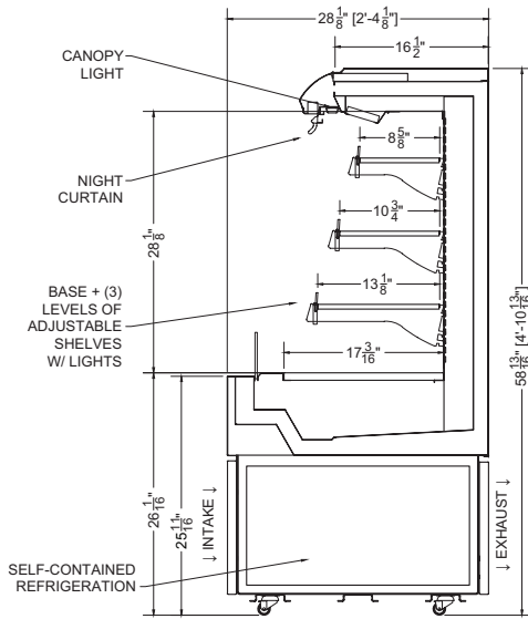
Section View
