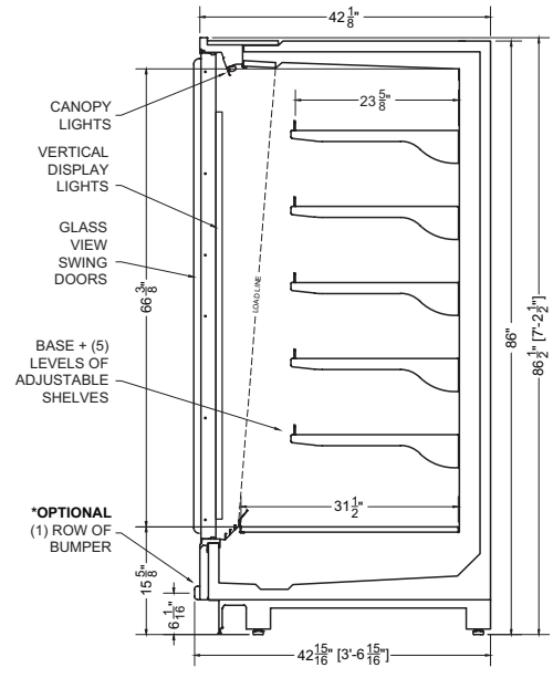
Section View
