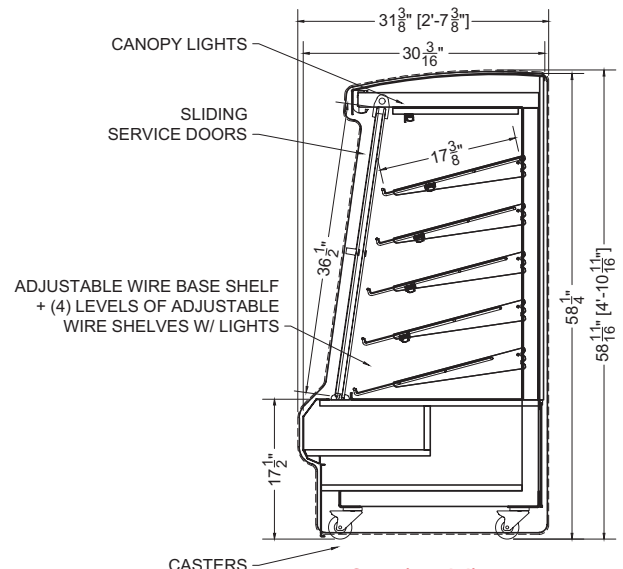
Section View
