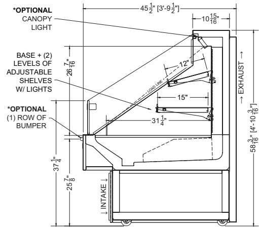
Section View
