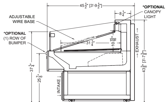
Section View
