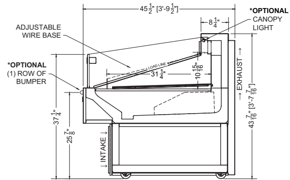
Section View
