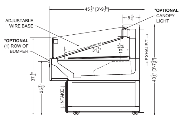
Section View
