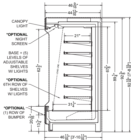
Section View
