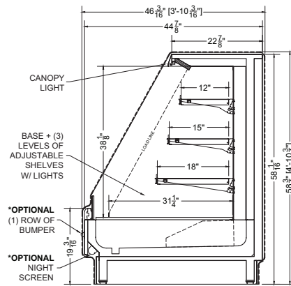
Section View
