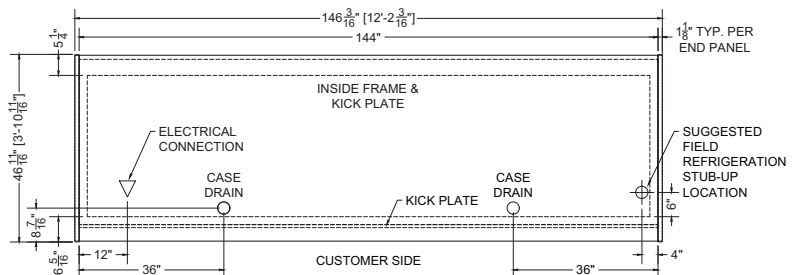
Plan Mechanical View
