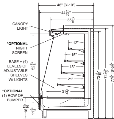
Section View
